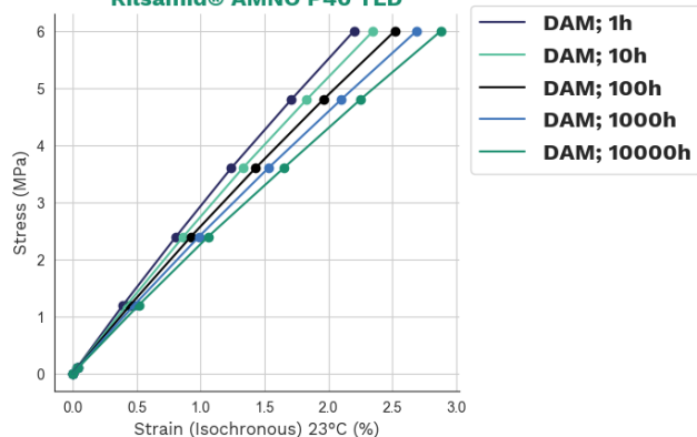
Stress-strain (isochronous) 23°C Rilsamid® AMNO P40 TLD
